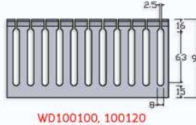
WD100100, 100120
