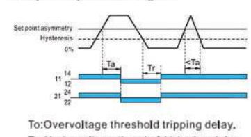
Asymmetry function diagram
