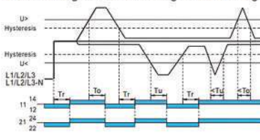
Overvoltage and undervoltage function diagram
